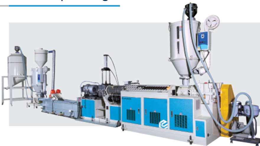
ABS Compounding
